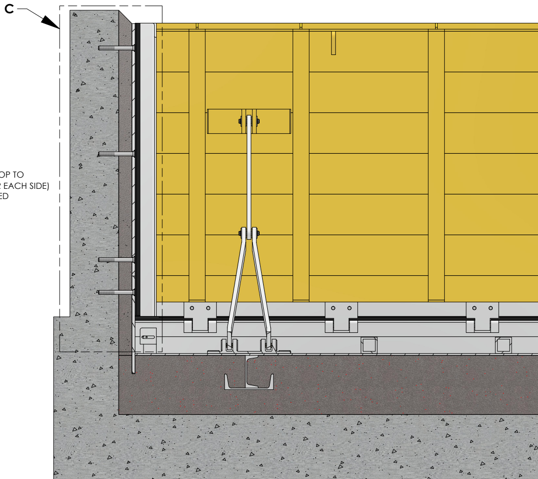
GATE LONGITUDINAL SECTION OPEN SECTION VIEW FROM WET SIDE CROPPED FOR CLARITY
