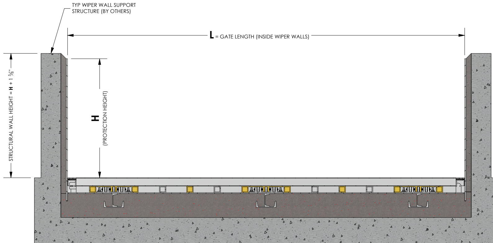
LONGITUDINAL SECTION IN CLOSED POSITION (VIEW FROM WET SIDE)
